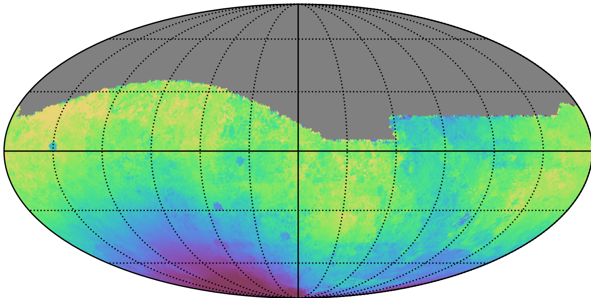
scp_reweight_v3.3_10yrs All sky g band: Median solarElong
