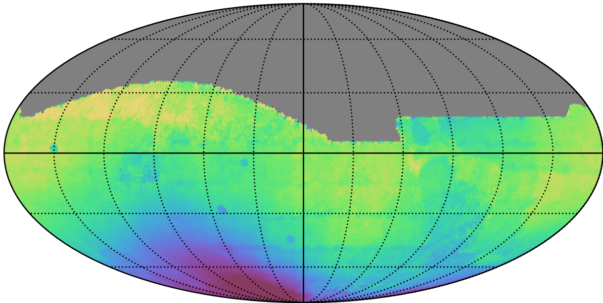
scp_reweight_v3.3_10yrs All sky all bands: Median solarElong
