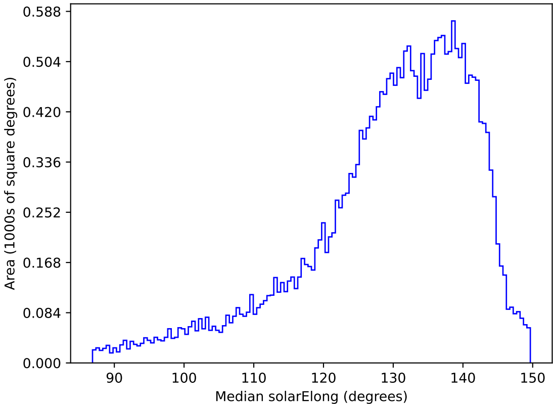
scp_reweight_v3.3_10yrs All sky all bands: Median solarElong
