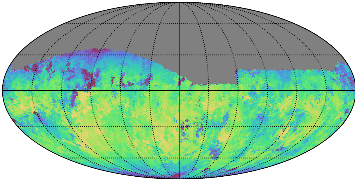
scp_reweight_v3.3_10yrs Yr 1 z band: Median skyBrightness
