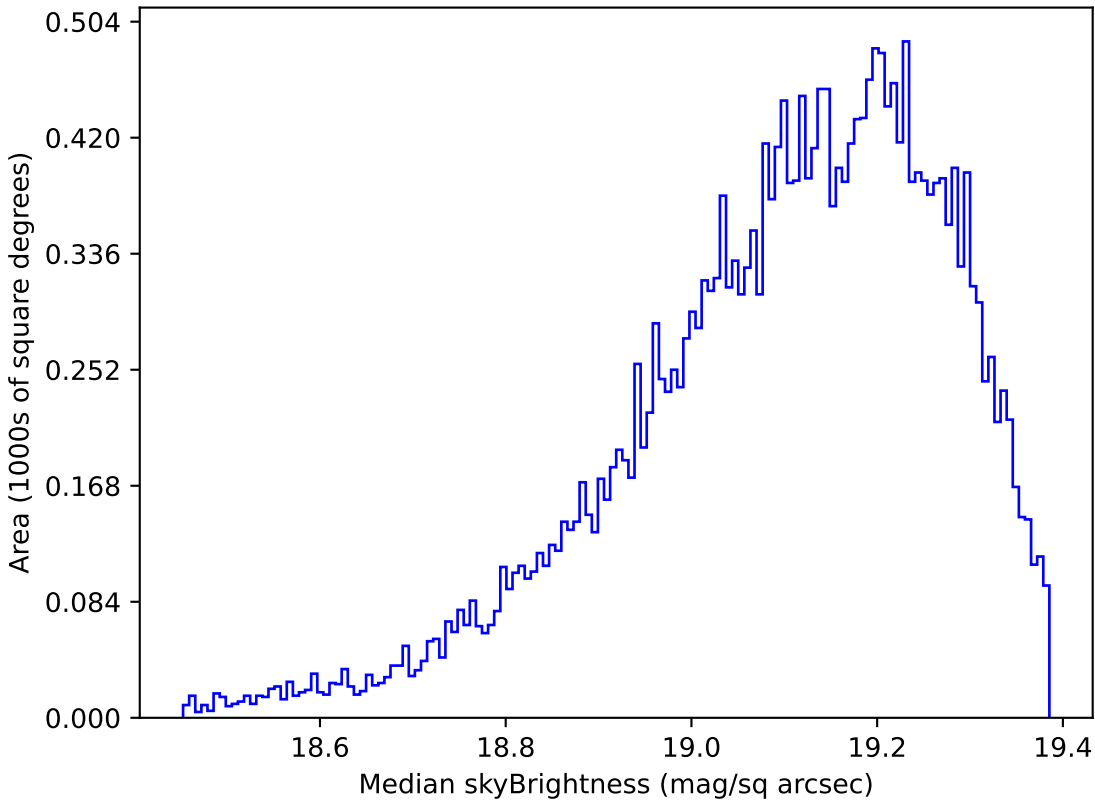
scp_reweight_v3.3_10yrs Yr 1 z band: Median skyBrightness
