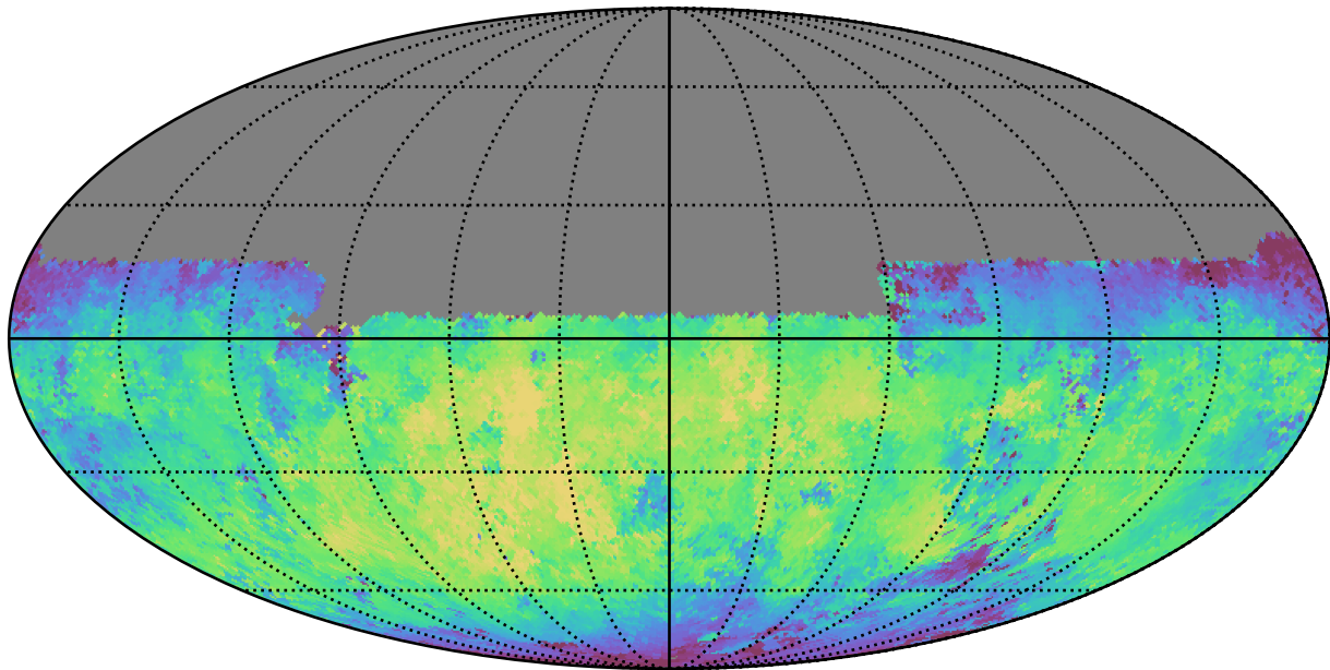
scp_reweight_v3.3_10yrs Yr 1 y band: Median skyBrightness
