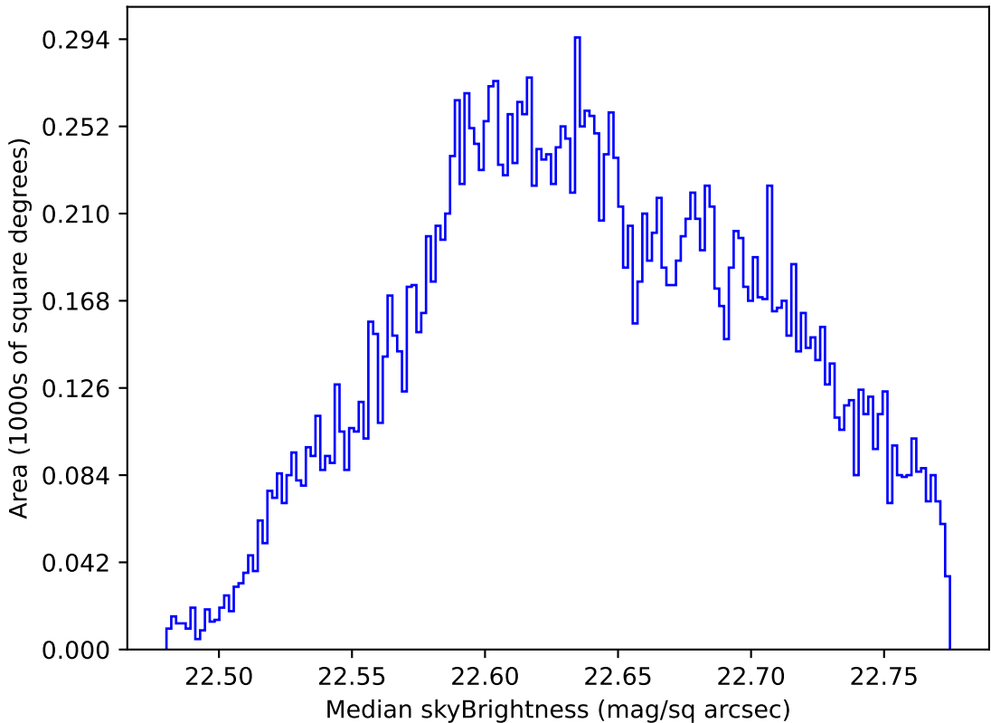
scp_reweight_v3.3_10yrs Yr 1 u band: Median skyBrightness
