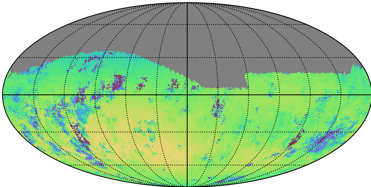
scp_reweight_v3.3_10yrs Yr 1 r band: Median skyBrightness
