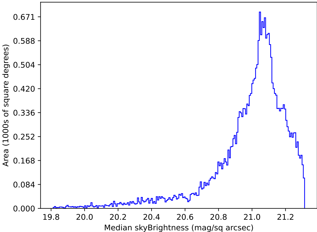
scp_reweight_v3.3_10yrs Yr 1 r band: Median skyBrightness
