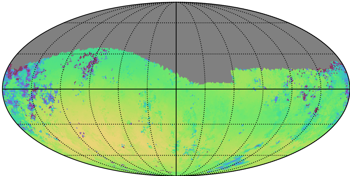
scp_reweight_v3.3_10yrs Yr 1 g band: Median skyBrightness
