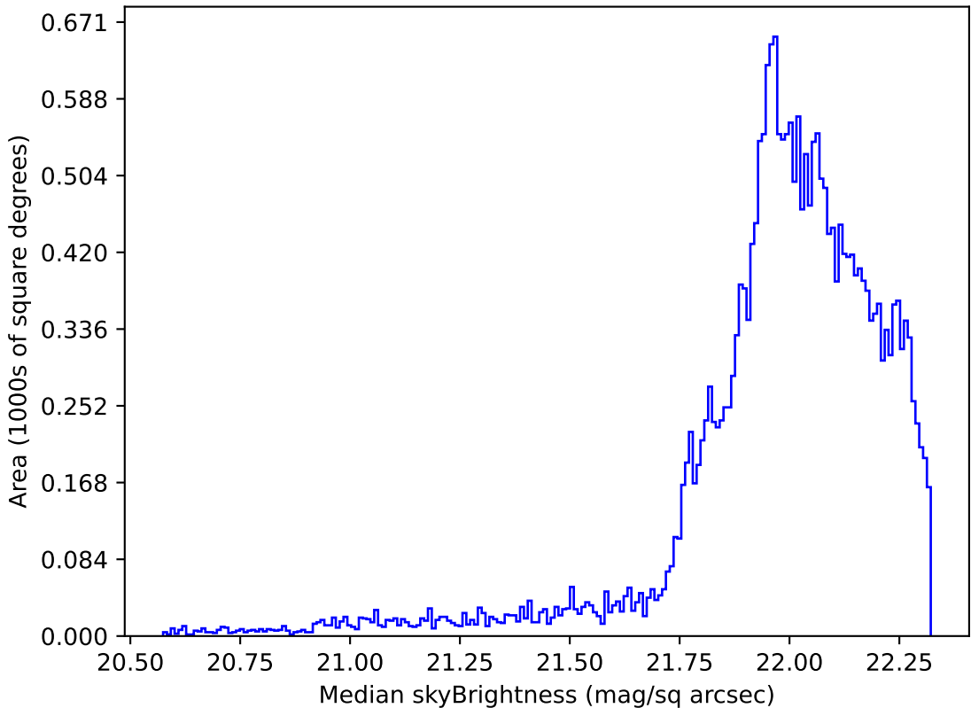
scp_reweight_v3.3_10yrs Yr 1 g band: Median skyBrightness
