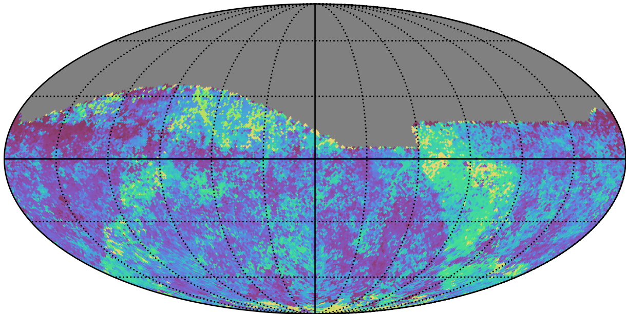
scp_reweight_v3.3_10yrs Yr 1 all bands: Median skyBrightness
