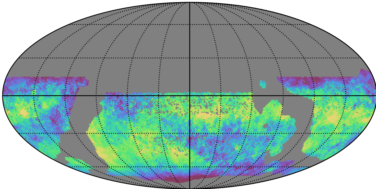
scp_reweight_v3.3_10yrs WFD z band: Median skyBrightness
