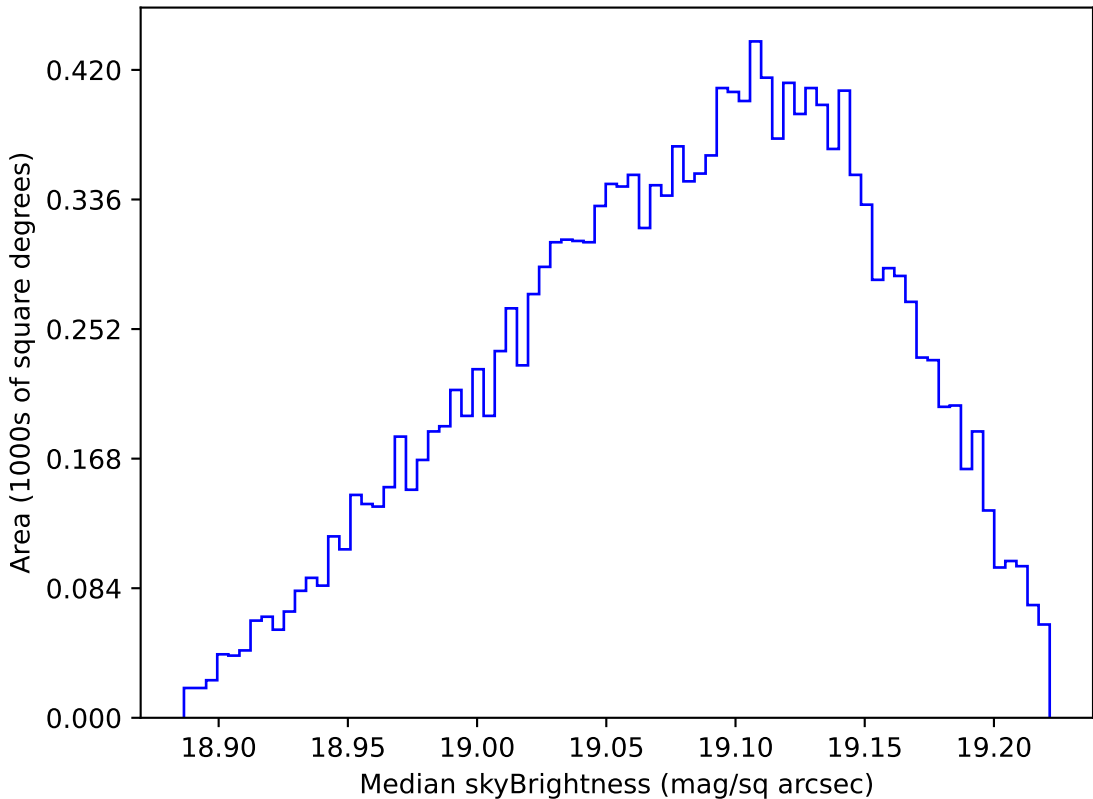
scp_reweight_v3.3_10yrs WFD z band: Median skyBrightness
