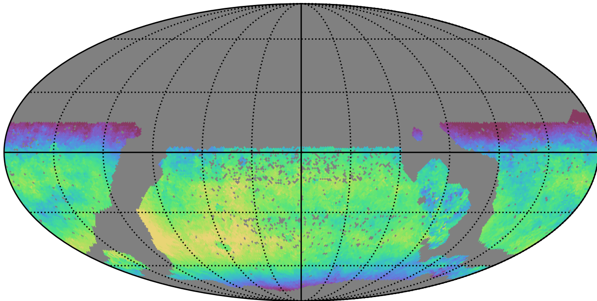
scp_reweight_v3.3_10yrs WFD y band: Median skyBrightness
