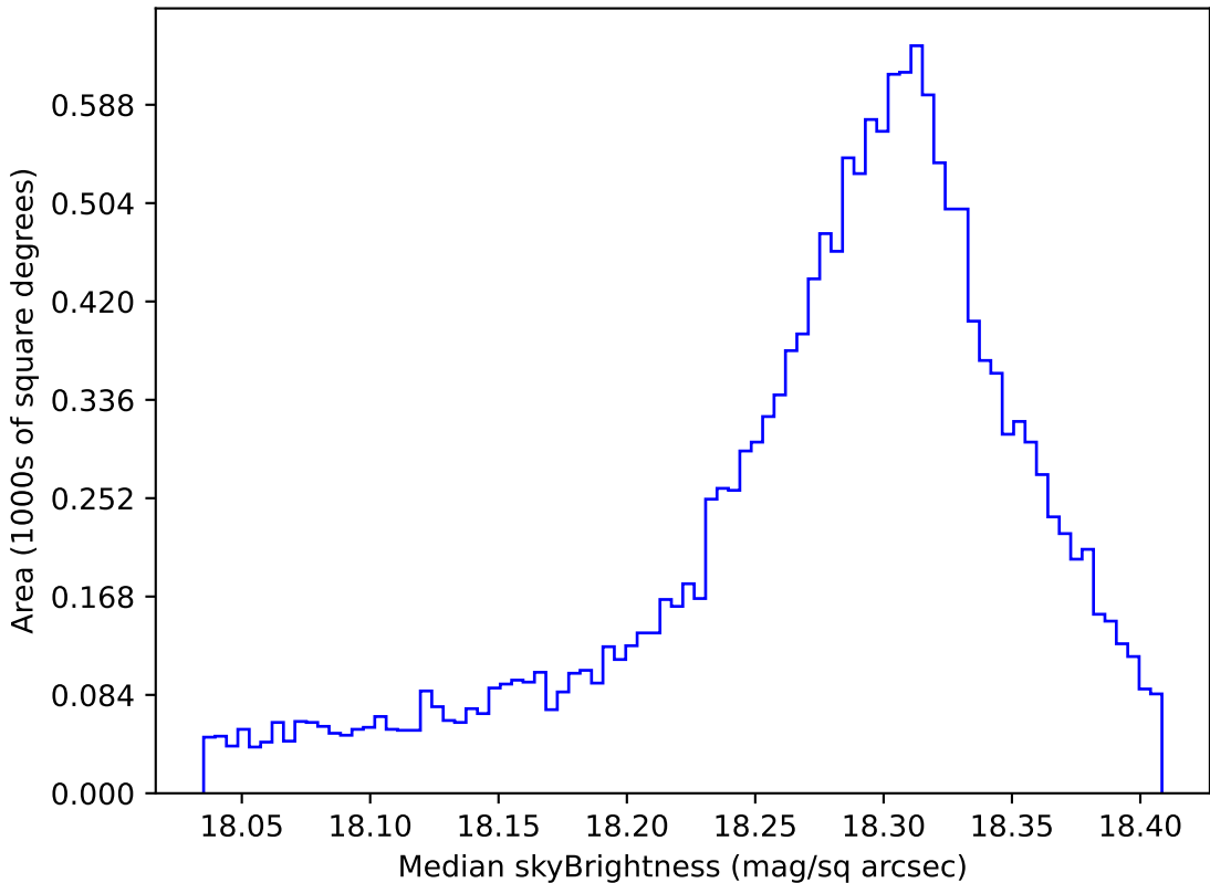
scp_reweight_v3.3_10yrs WFD y band: Median skyBrightness
