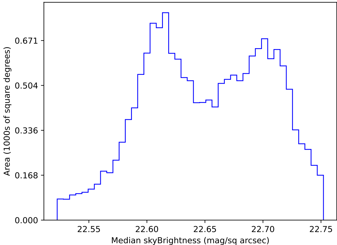
scp_reweight_v3.3_10yrs WFD u band: Median skyBrightness
