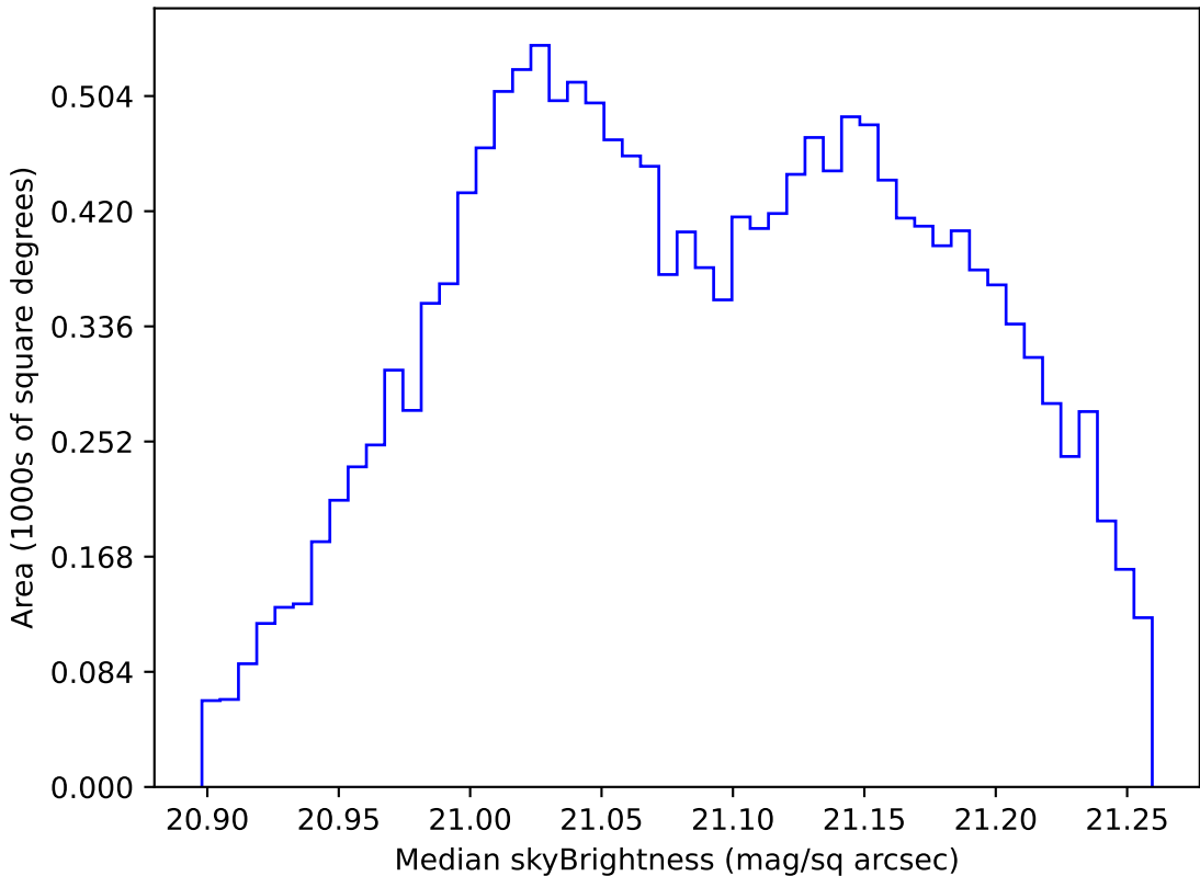
scp_reweight_v3.3_10yrs WFD r band: Median skyBrightness
