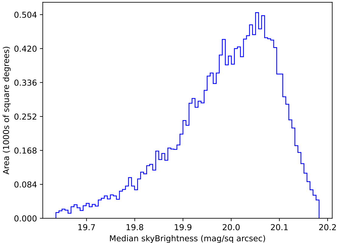
scp_reweight_v3.3_10yrs WFD i band: Median skyBrightness
