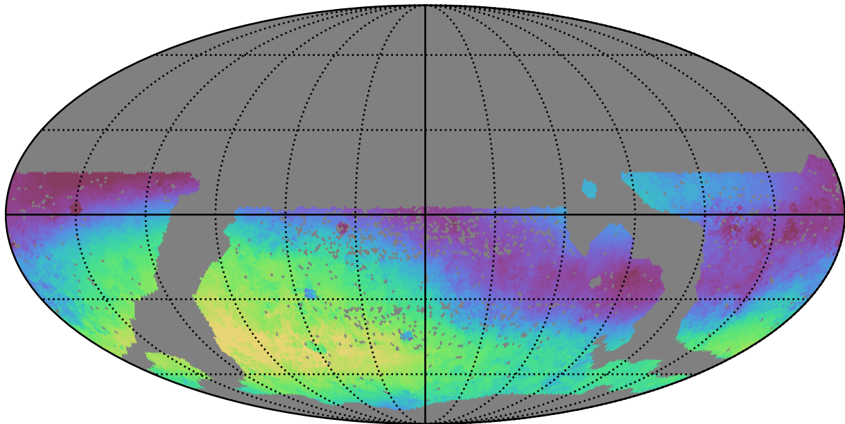
scp_reweight_v3.3_10yrs WFD g band: Median skyBrightness
