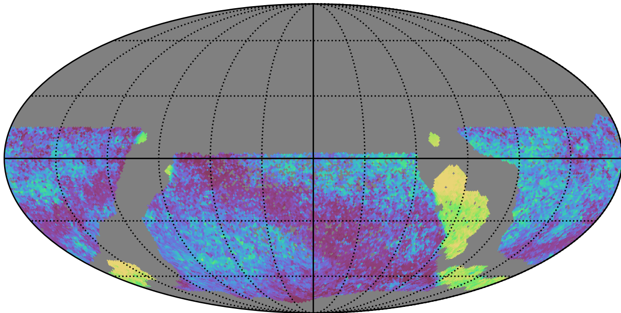
scp_reweight_v3.3_10yrs WFD all bands: Median skyBrightness
