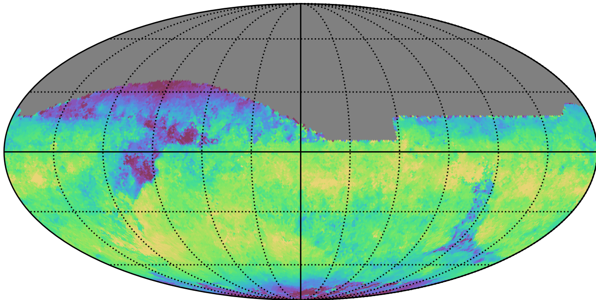
scp_reweight_v3.3_10yrs All sky z band: Median skyBrightness
