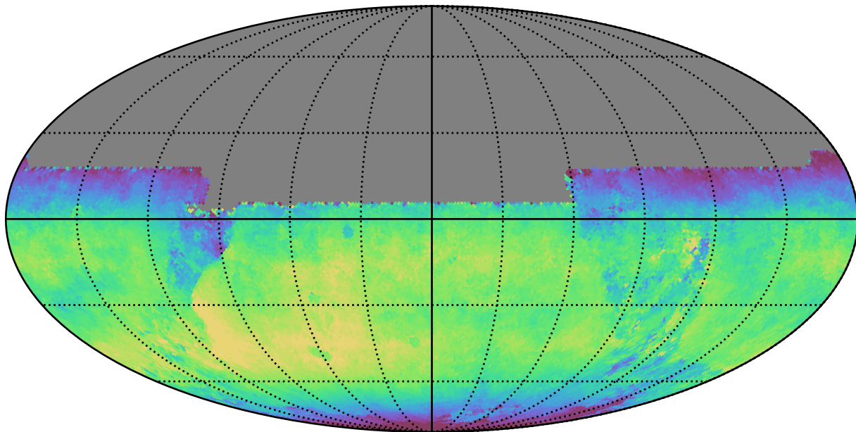
scp_reweight_v3.3_10yrs All sky y band: Median skyBrightness
