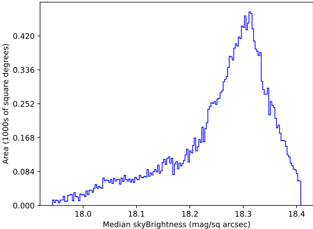
scp_reweight_v3.3_10yrs All sky y band: Median skyBrightness
