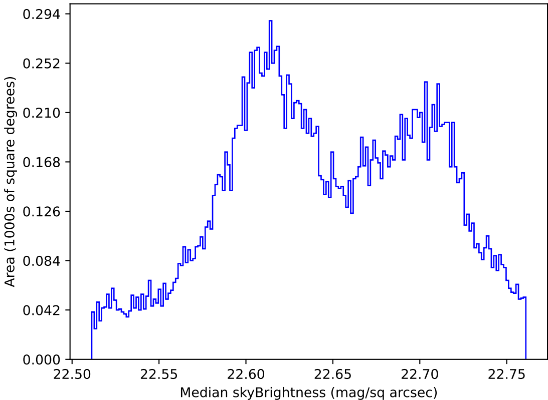
scp_reweight_v3.3_10yrs All sky u band: Median skyBrightness
