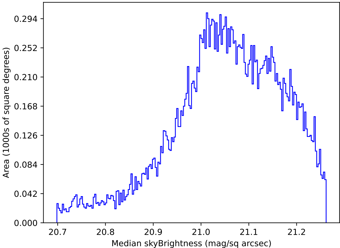
scp_reweight_v3.3_10yrs All sky r band: Median skyBrightness
