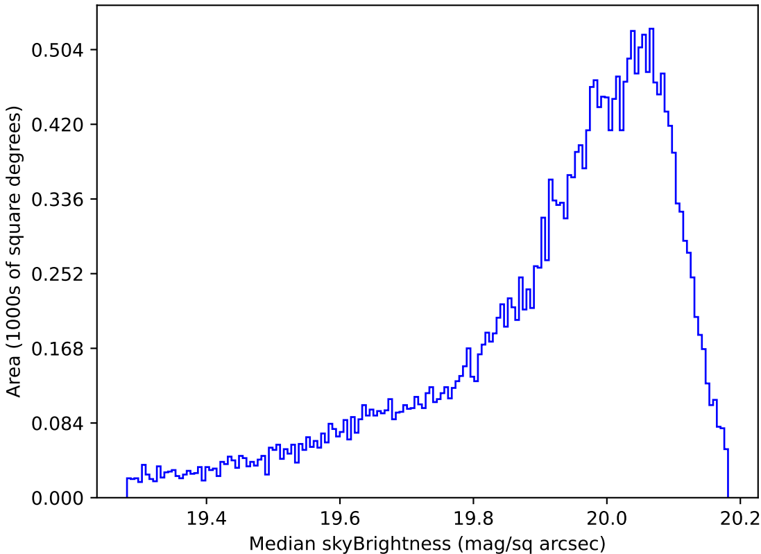
scp_reweight_v3.3_10yrs All sky i band: Median skyBrightness
