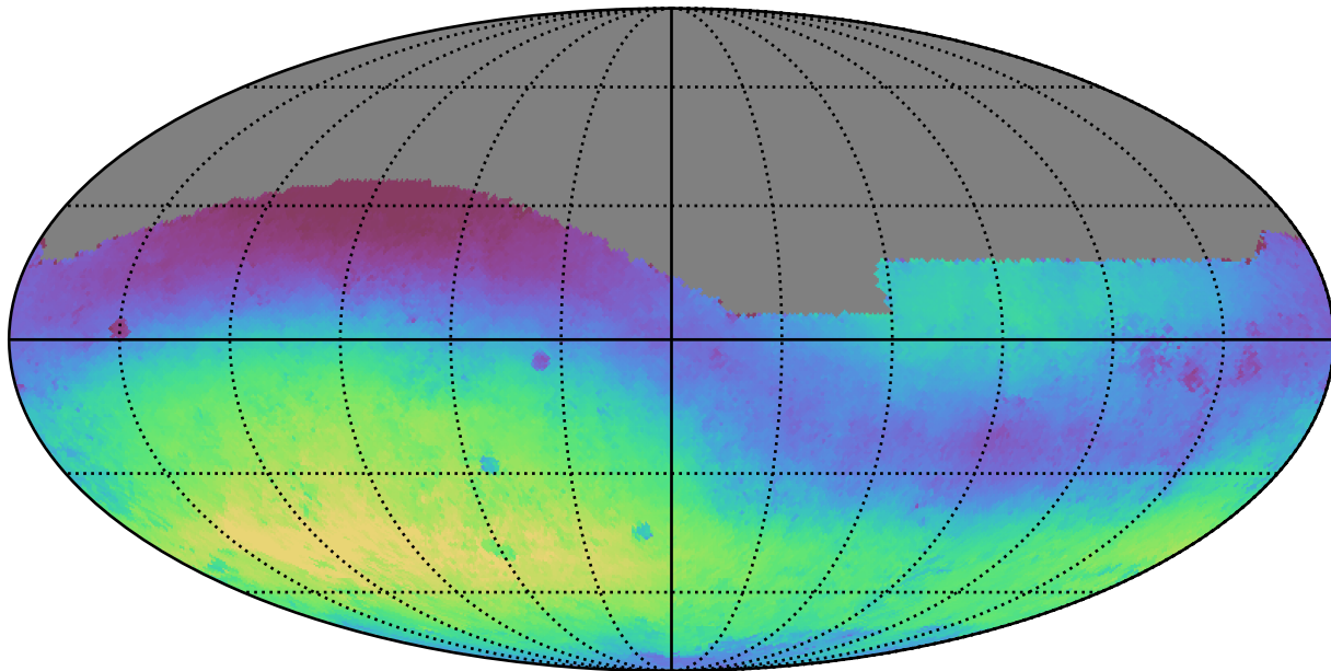
scp_reweight_v3.3_10yrs All sky g band: Median skyBrightness
