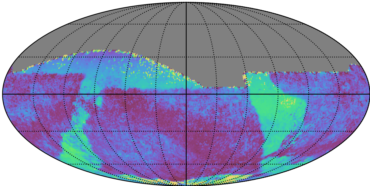
scp_reweight_v3.3_10yrs All sky all bands: Median skyBrightness
