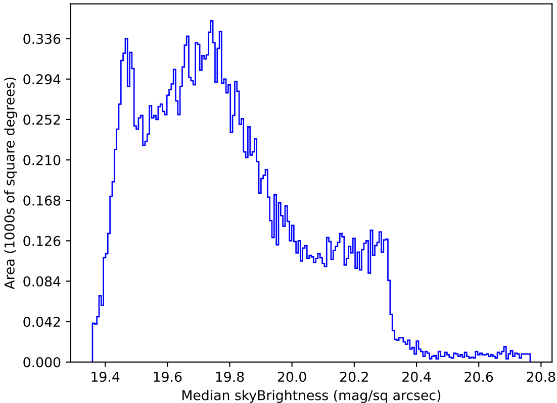
scp_reweight_v3.3_10yrs All sky all bands: Median skyBrightness
