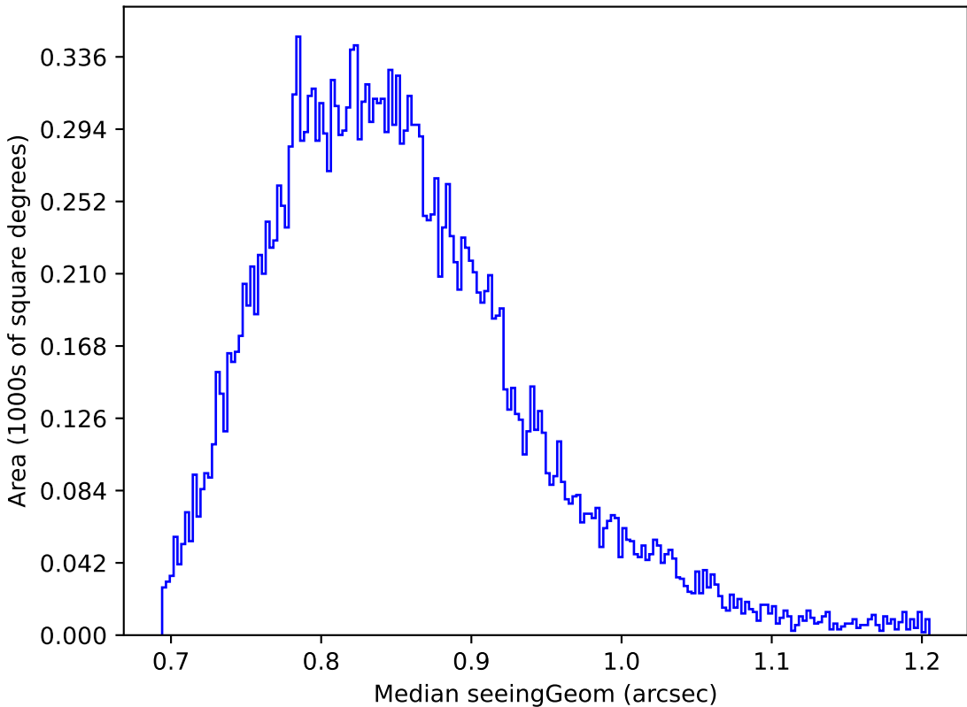
scp_reweight_v3.3_10yrs Yr 1 y band: Median seeingGeom
