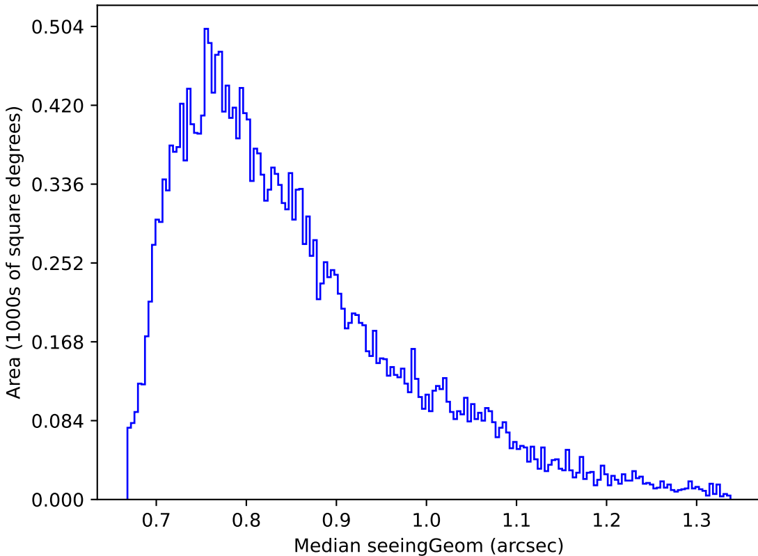
scp_reweight_v3.3_10yrs Yr 1 r band: Median seeingGeom
