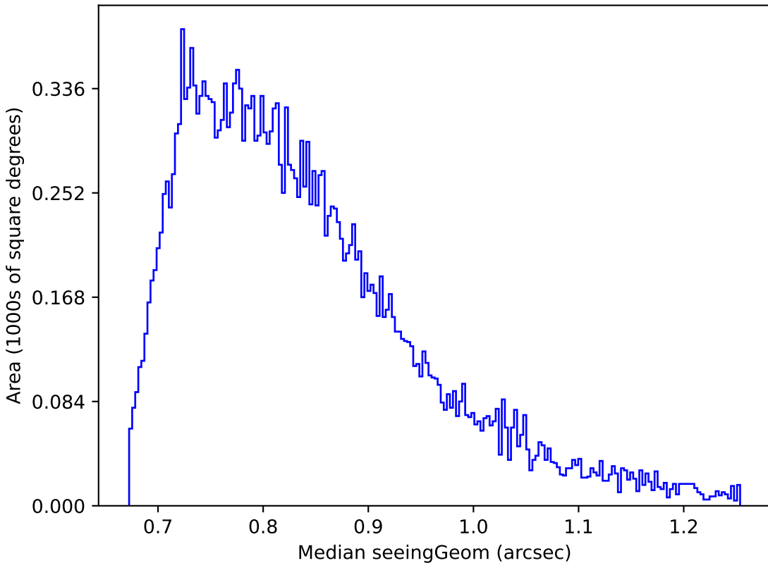
scp_reweight_v3.3_10yrs Yr 1 i band: Median seeingGeom
