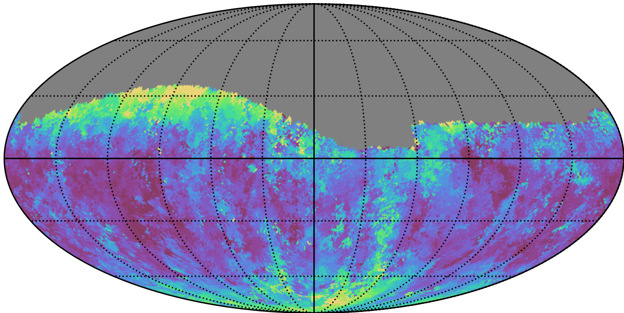
scp_reweight_v3.3_10yrs Yr 1 g band: Median seeingGeom
