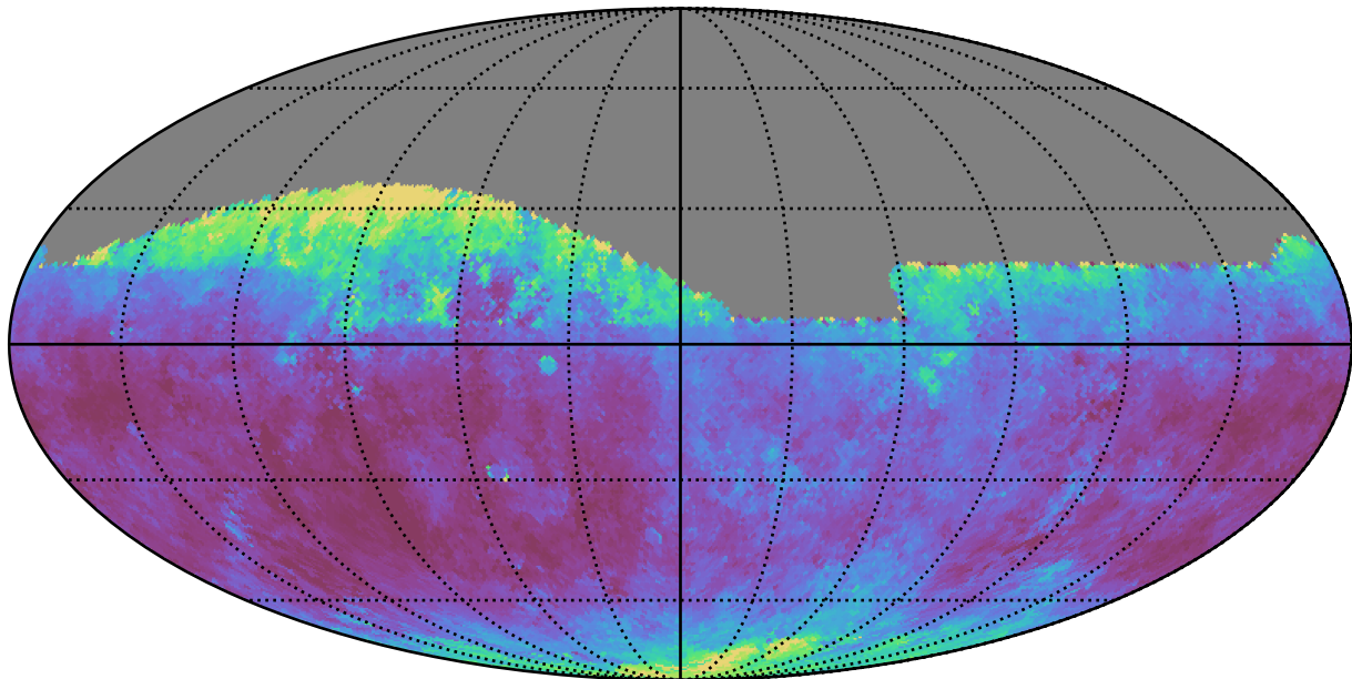
scp_reweight_v3.3_10yrs Yr 1 all bands: Median seeingGeom
