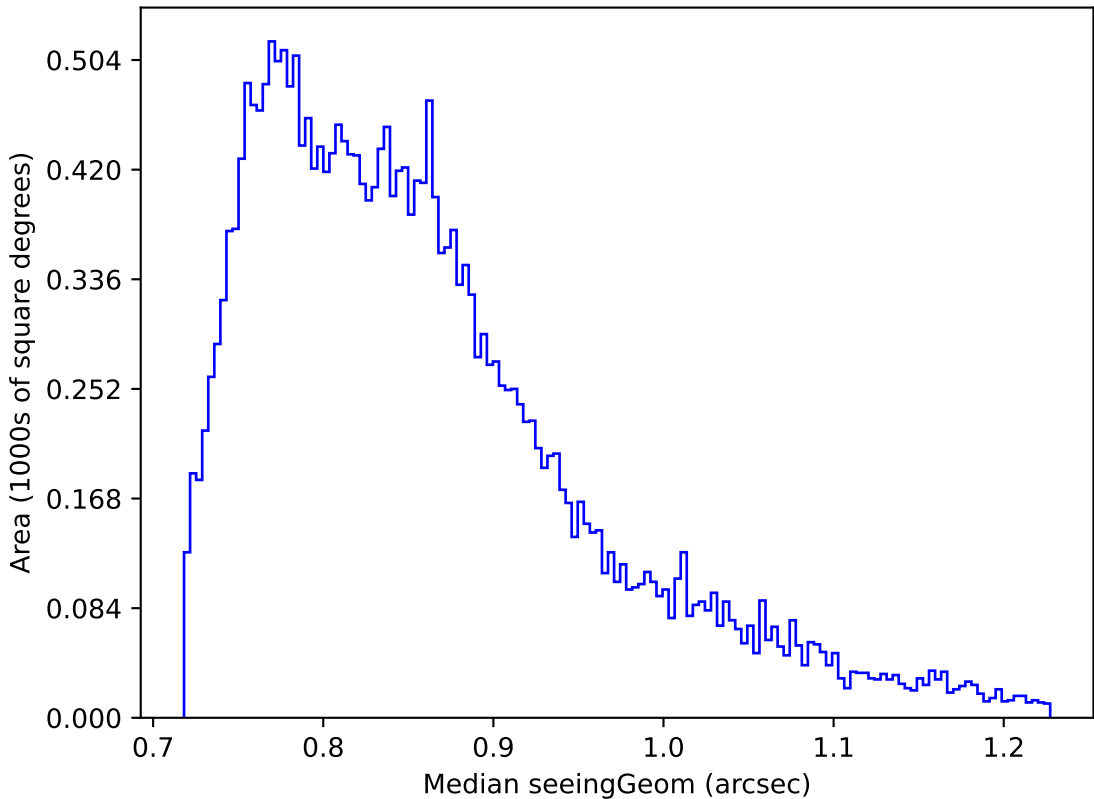
scp_reweight_v3.3_10yrs Yr 1 all bands: Median seeingGeom
