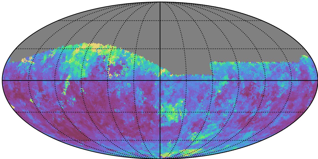
scp_reweight_v3.3_10yrs Yr1 z band: Median seeingEff
