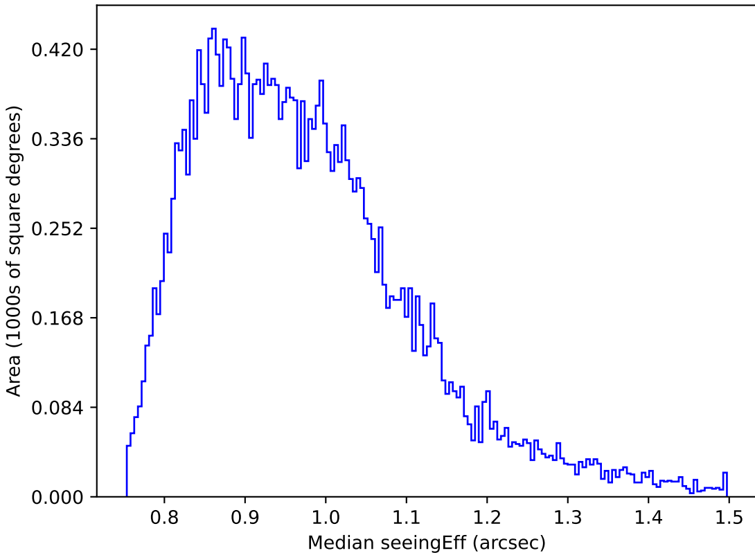
scp_reweight_v3.3_10yrs Yr 1 z band: Median seeingEff
