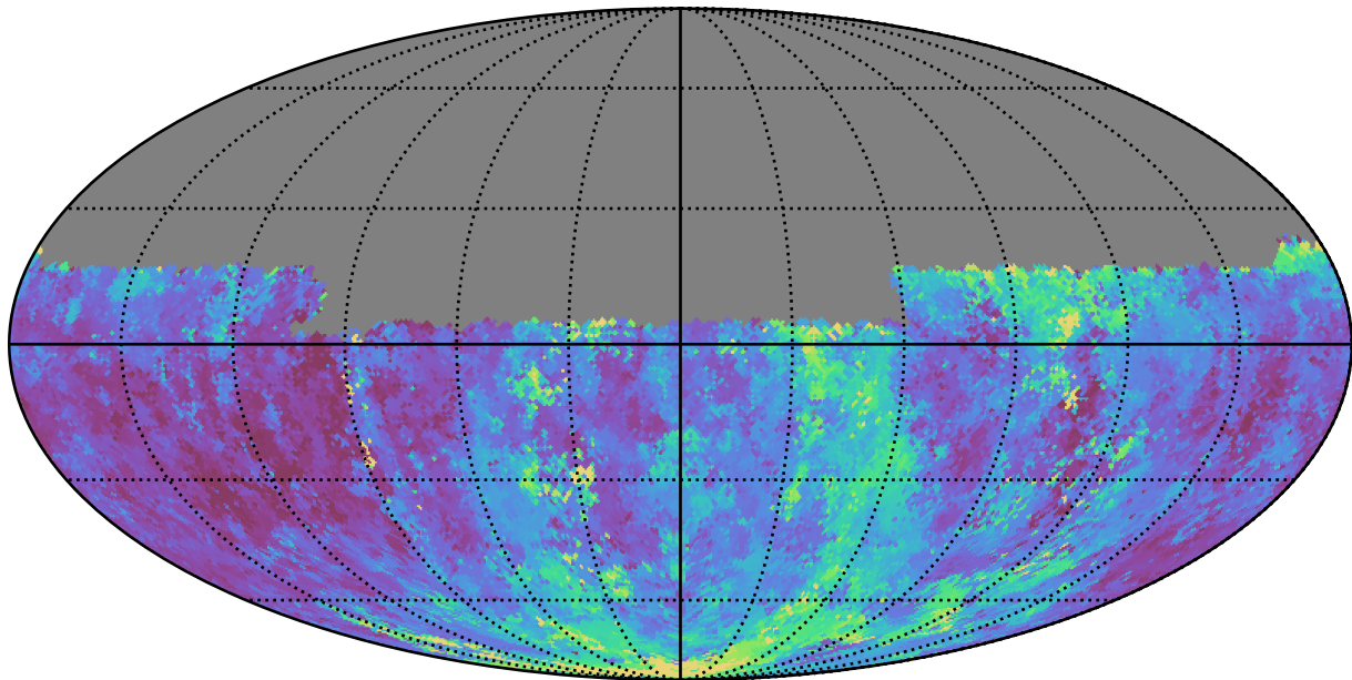
scp_reweight_v3.3_10yrs Yr 1 u band: Median seeingEff
