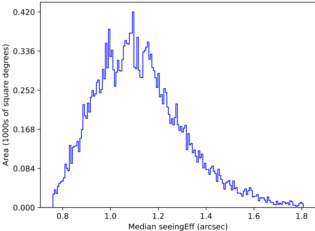
scp_reweight_v3.3_10yrs Yr 1 u band: Median seeingEff
