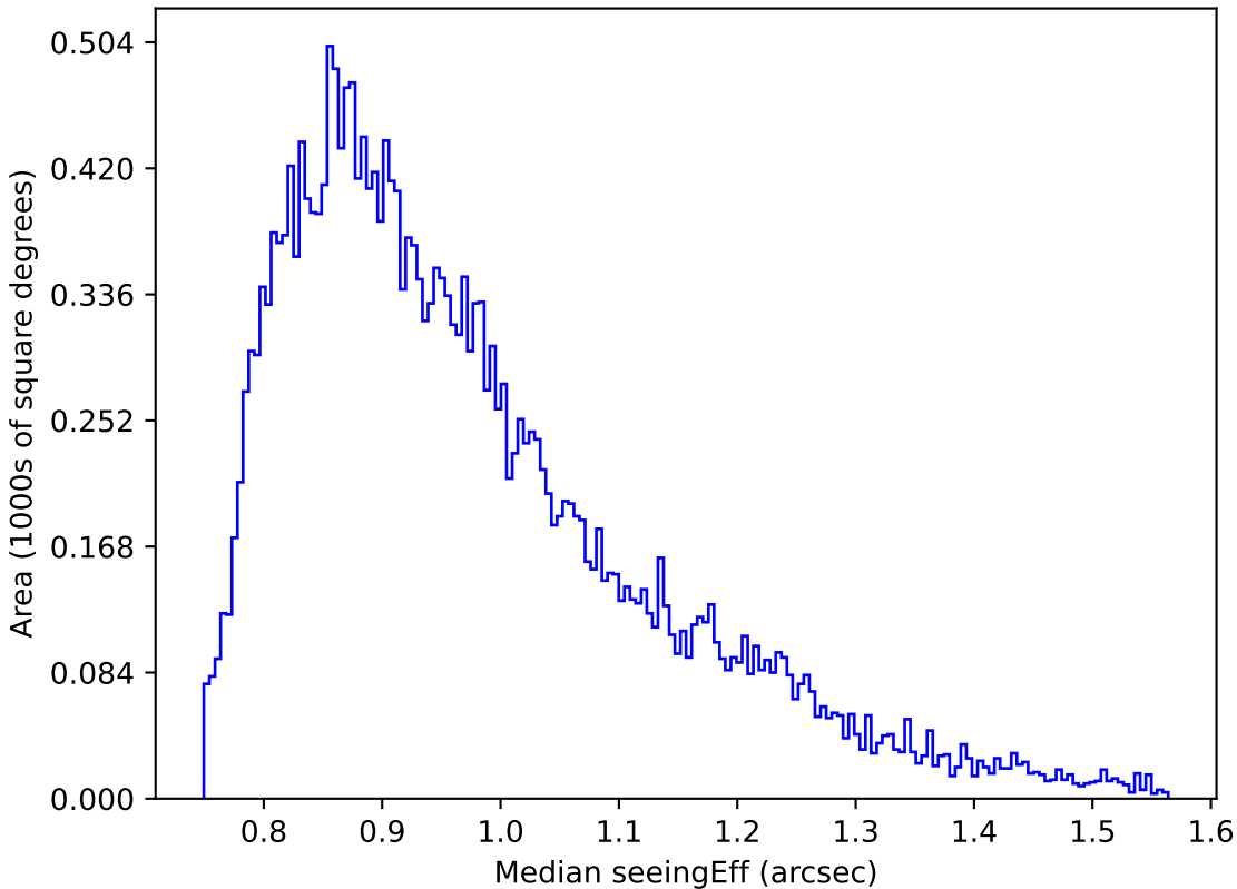
scp_reweight_v3.3_10yrs Yr 1 r band: Median seeingEff
