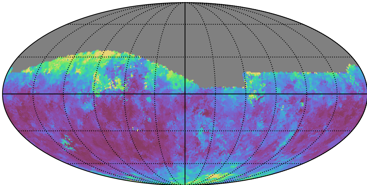
scp_reweight_v3.3_10yrs Yr 1 i band: Median seeingEff
