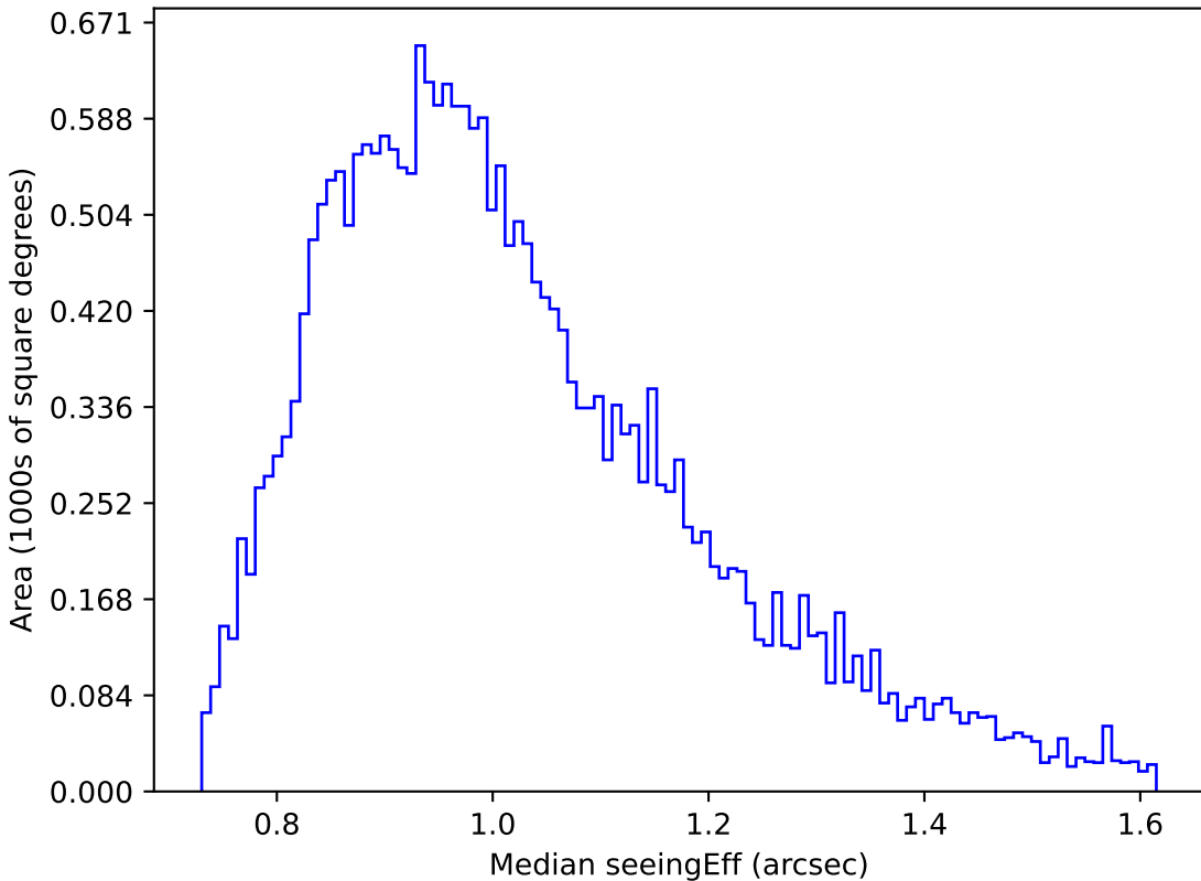
scp_reweight_v3.3_10yrs Yr 1 g band: Median seeingEff
