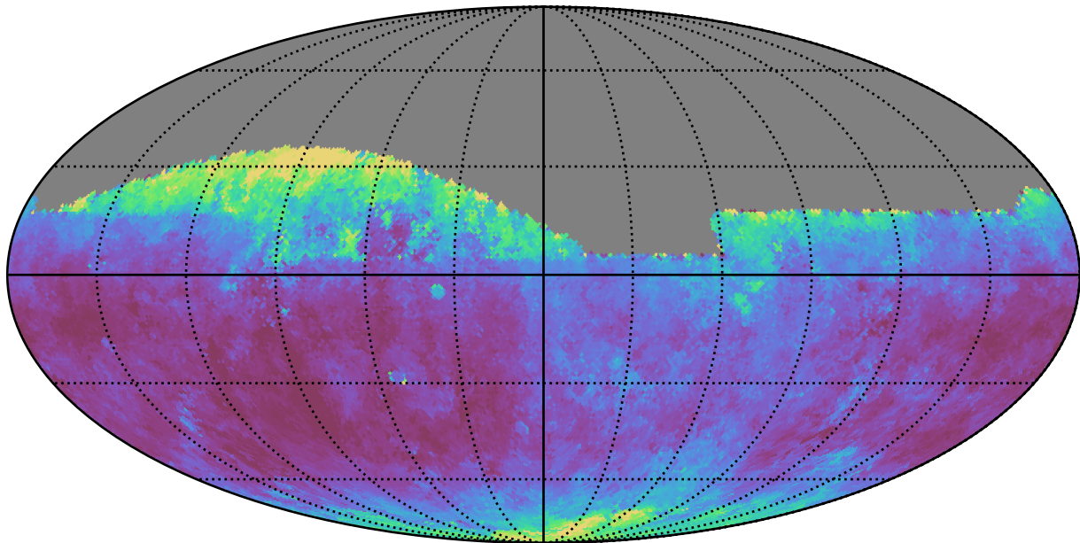
scp_reweight_v3.3_10yrs Yr 1 all bands: Median seeingEff
