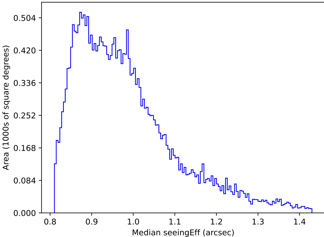
scp_reweight_v3.3_10yrs Yr 1 all bands: Median seeingEff
