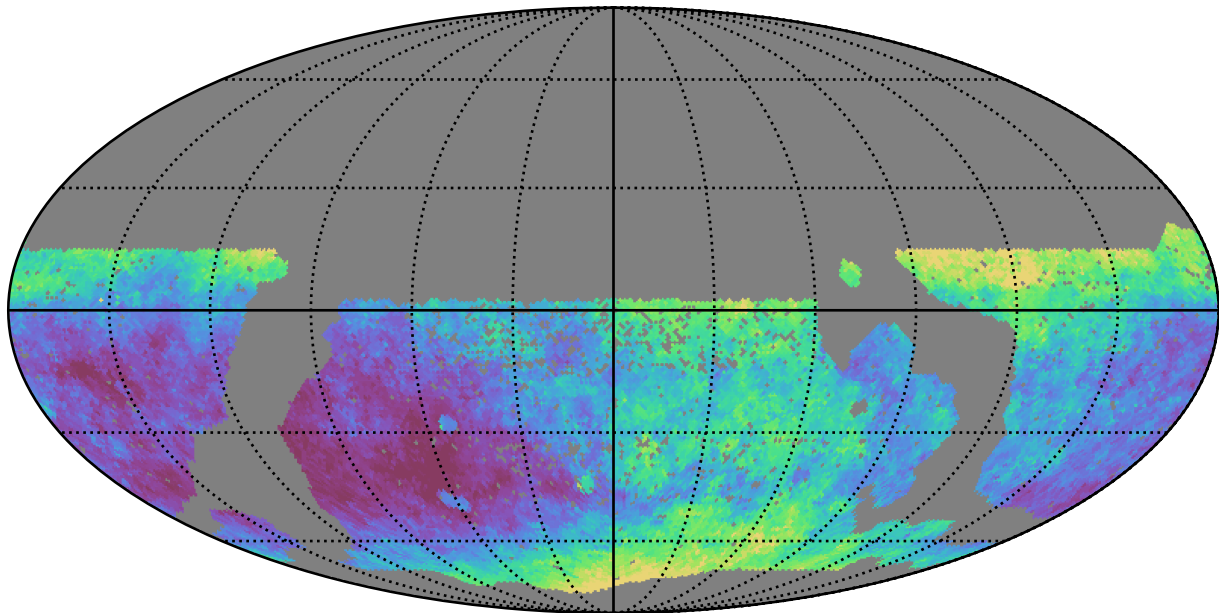
scp_reweight_v3.3_10yrs WFD z band: Median seeingEff
