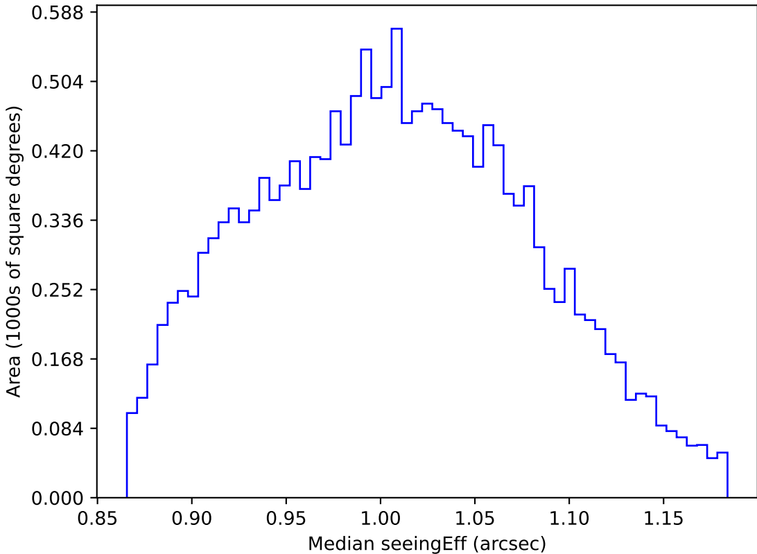
scp_reweight_v3.3_10yrs WFD z band: Median seeingEff
