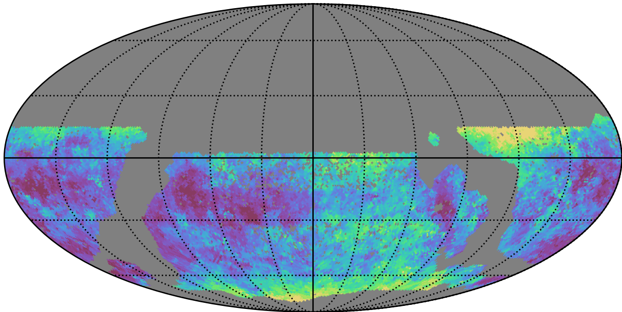
scp_reweight_v3.3_10yrs WFD u band: Median seeingEff
