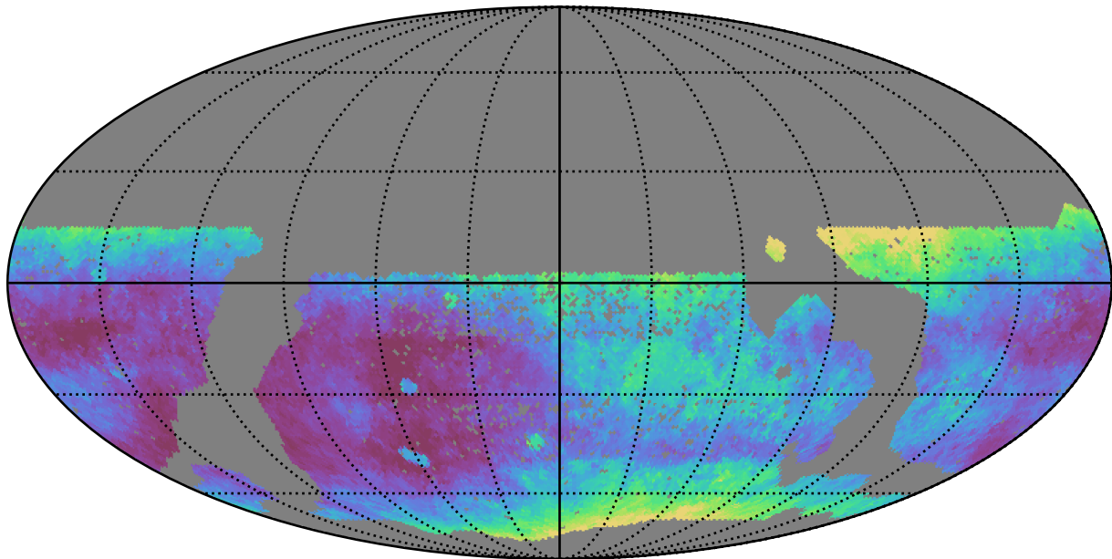
scp_reweight_v3.3_10yrs WFD r band: Median seeingEff
