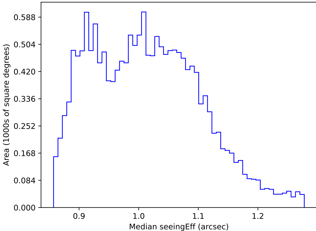
scp_reweight_v3.3_10yrs WFD r band: Median seeingEff
